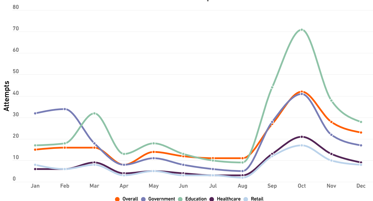
2020 IoT Malware Attempts Per Customer
