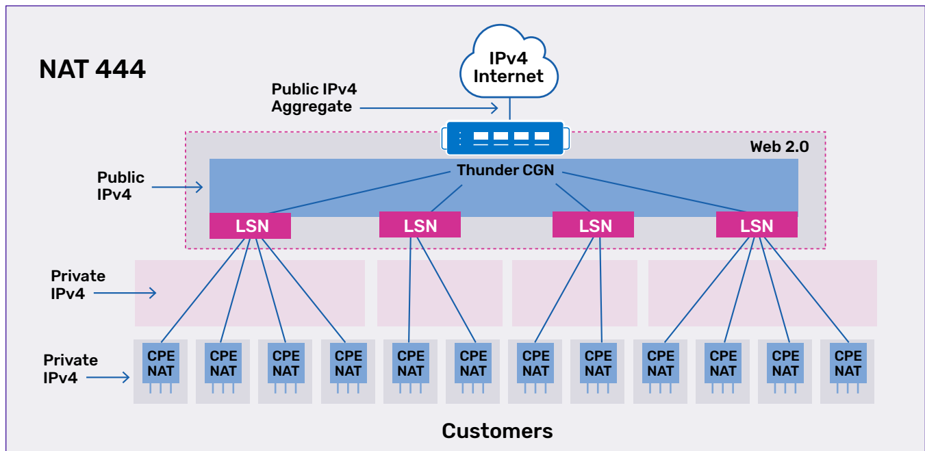
Figure 1: NAT 444/CGN - A Triple NAT (IPv4 to IPv4 to IPv4)
